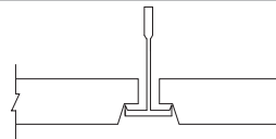
SHADOWLINE TEGULAR (SLT)
