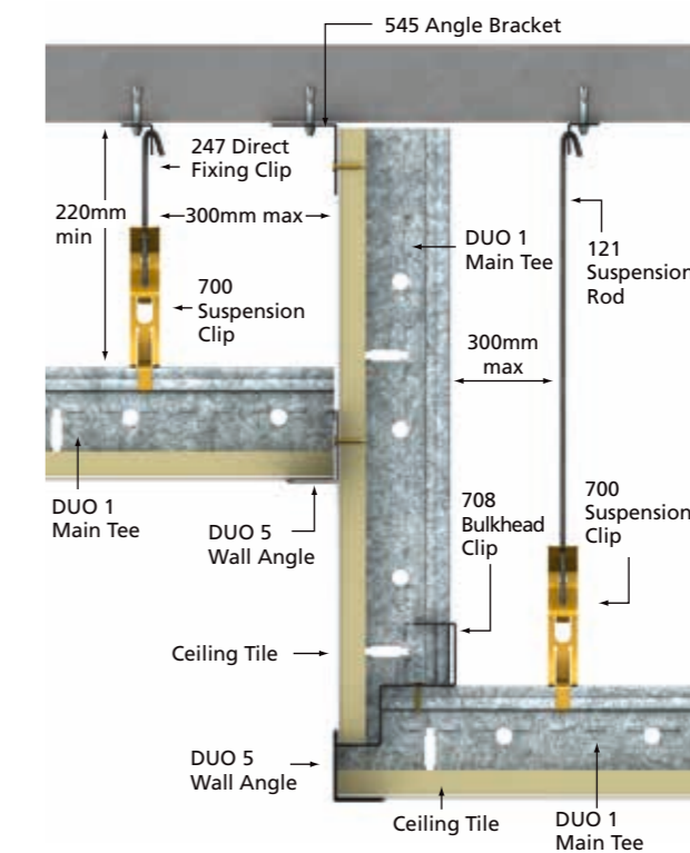
FIGURE 8: SQUARELINE BULKHEAD DETAIL (VERTICAL EXPOSED GRID)
