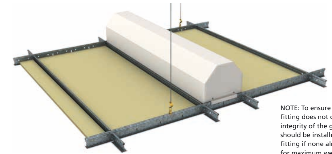
FIGURE 7: LIGHT FITTING DETAIL
